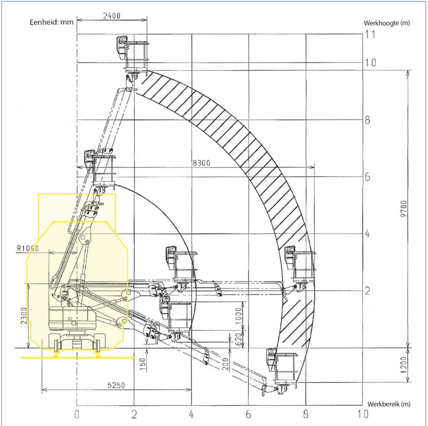
Profile of free space of the Hitachi HX99B.
